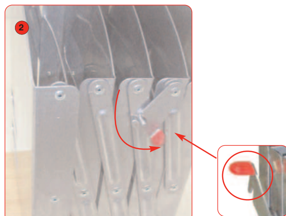
Push locking arm backwards to release
