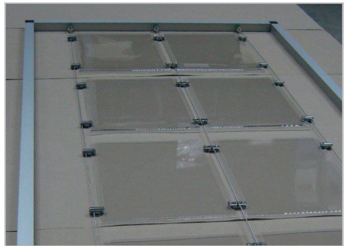
Mounting of acrylic U-pockets
