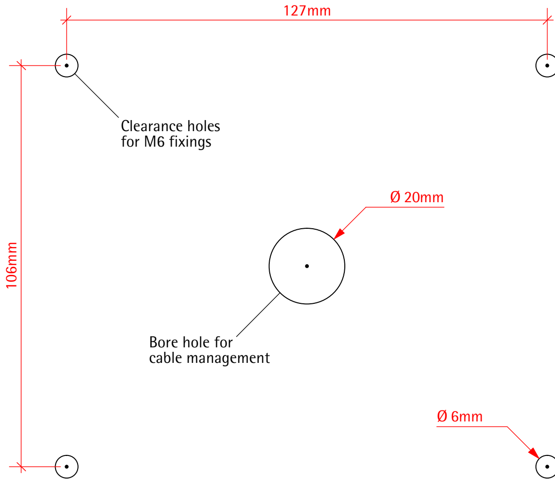
Template for optional screw mounting
