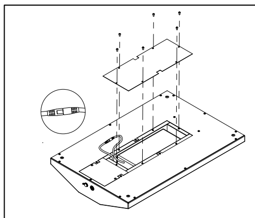
Schematic diagram of battery pack replacement
